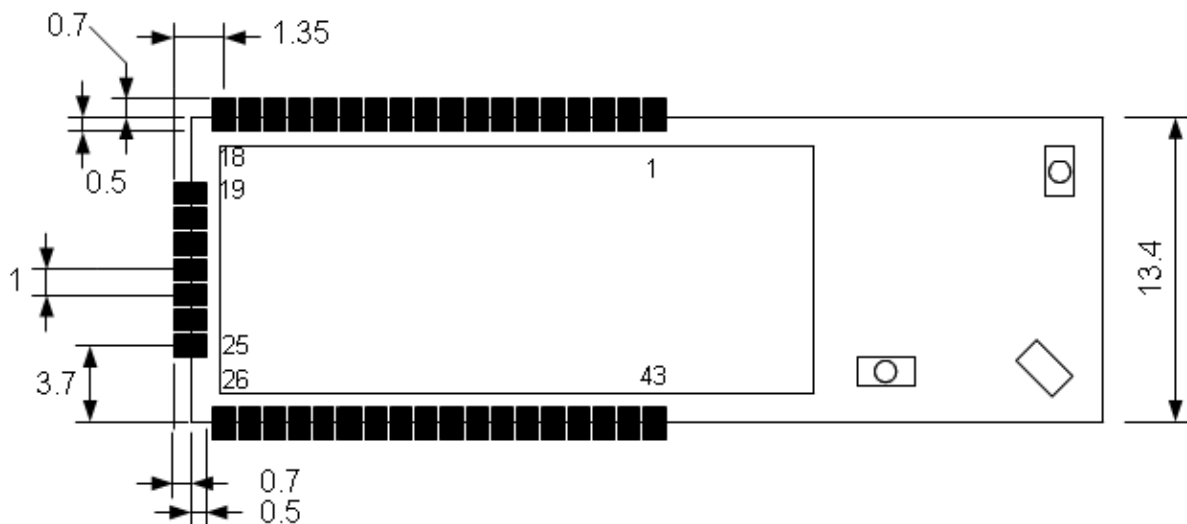
Figure 3 Footprint description for PCB layout
